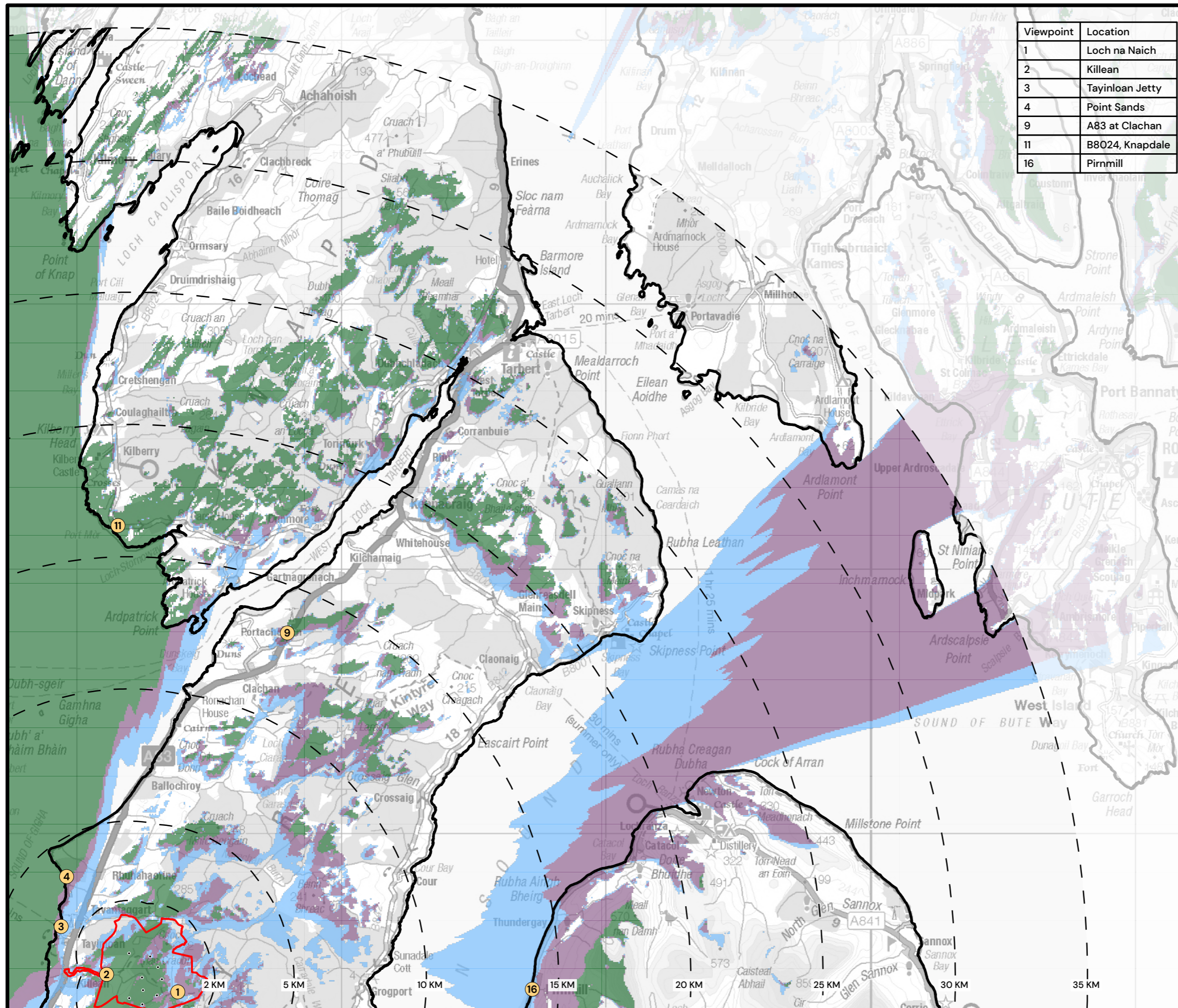
FIGURE 5.25 HUB HEIGHT ZTV TO 35 KM (NE QUADRANT) AND VIEWPOINTS
