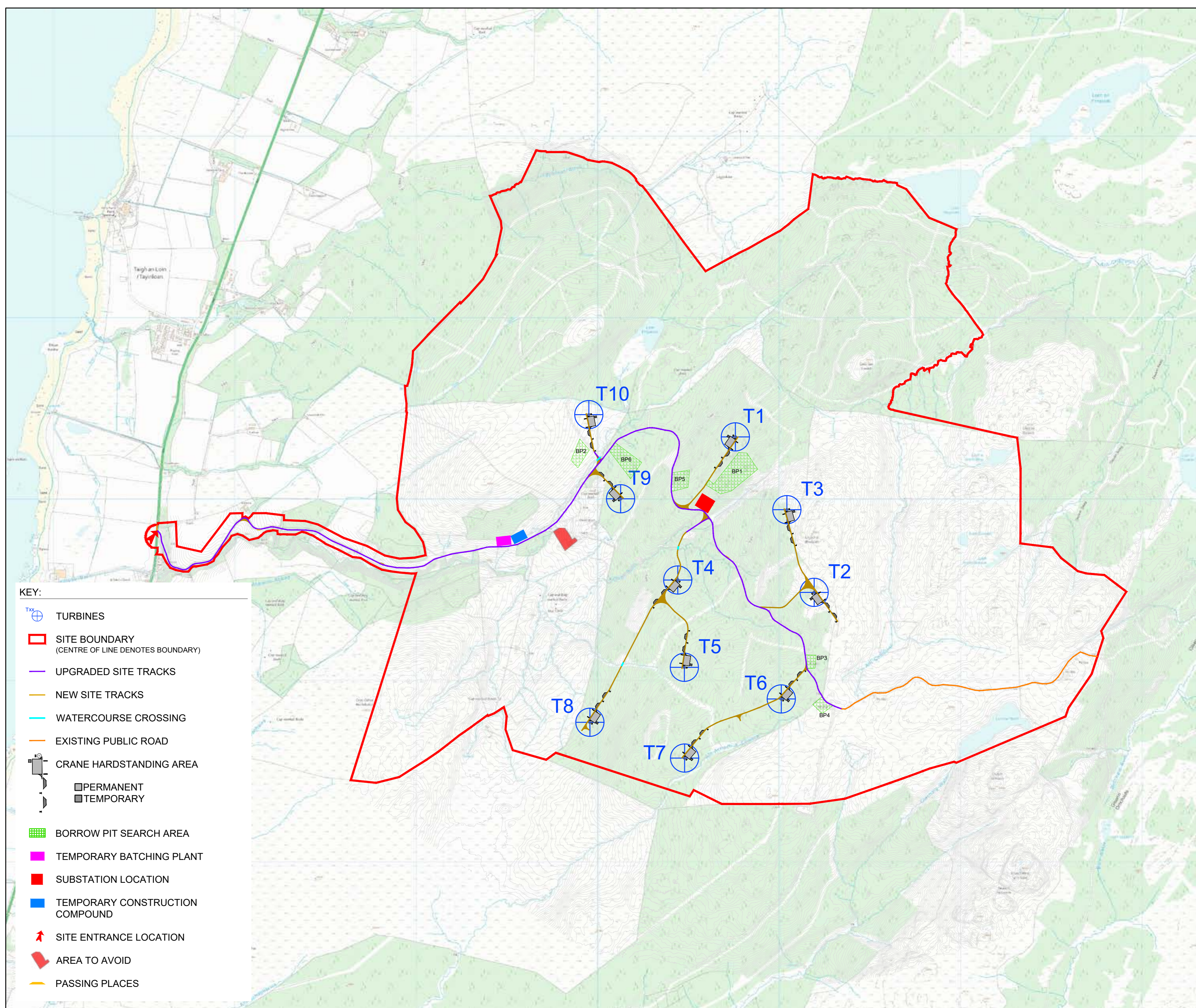
Infrastructure layout
